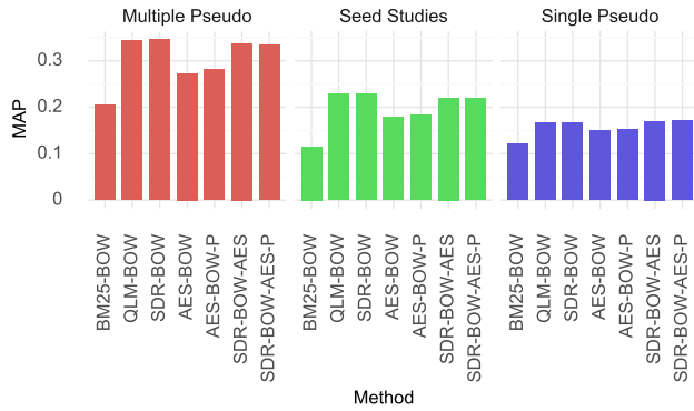
Figure 4: Comparison between the different arrangements of seed and pseudo-seed studies across the SDR methods. We have chosen to show only MAP, but all evaluation measures we chose showed the same trend.
