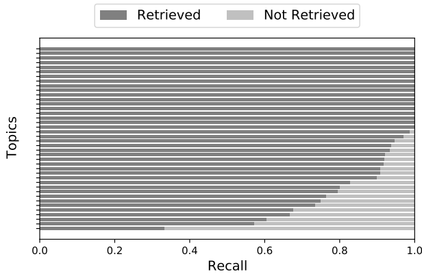
Figure 3: Recall distribution of all of the topics given the combined set of studies that includes retrieved studies, the seed-snowballed set, and the screened-snowballed set.
